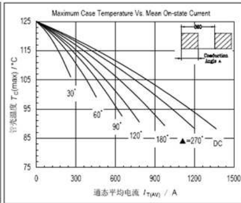
图6. 管壳温度与通态平均电流的关系曲线 Fig6 Case temperature range and Mean on-state current curve
