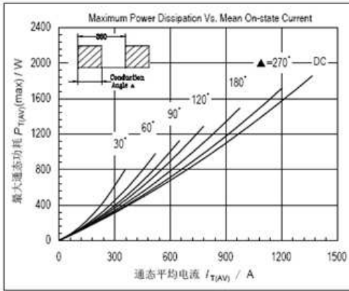
图5. 最大通态功耗与通态平均电流的关系曲线 Fig5 Maximum power consumption and Mean on-state current curve
