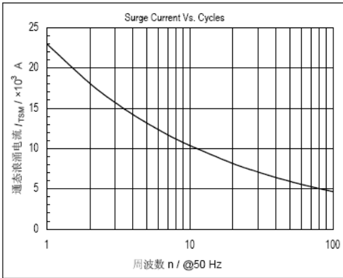
图7. 通态浪涌电流与周波数的关系曲线 Fig7. Surge on-state current and Cycle number
