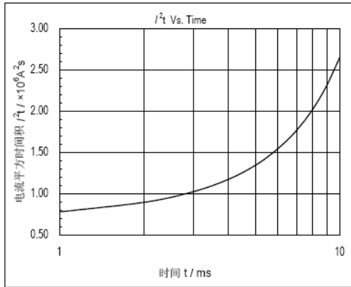
图8. I 2 t 特性曲线 Fig8. I 2 t characteristic curve
