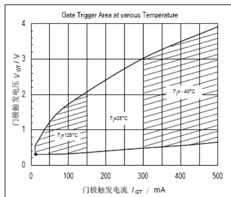
图10. 不同结温下的门极触发区 Fig10. Different junction temperature of the gate trigger area
